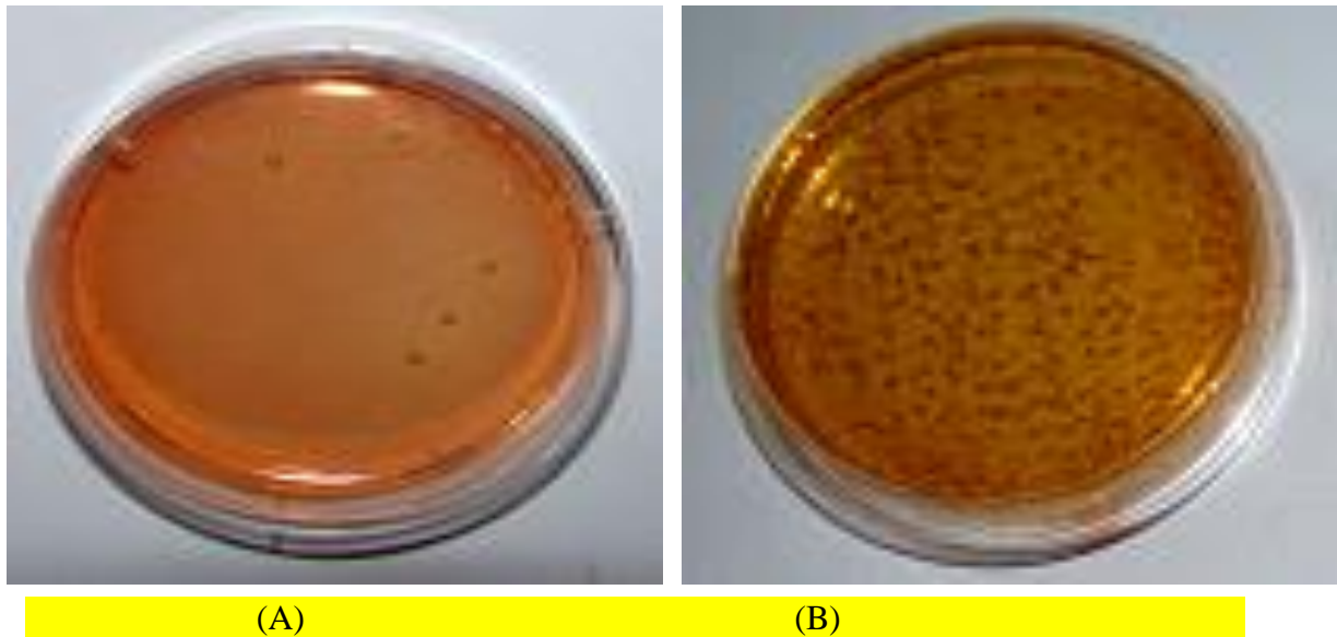
Fig(4): comparison between Salmonella Spp exposed and non exposed to superoxide radicals.
