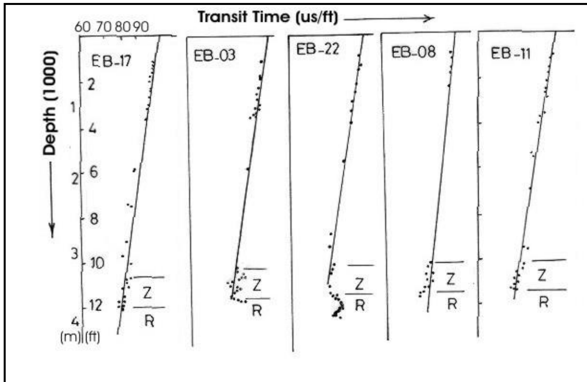
Fig. 8 : Shale transit time \Delta t with increasing depth in Zubair and Ratawi formations (wells 17, 3, 22, 8 and 11).
