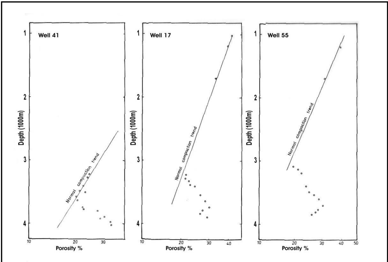
Fig. 5 : Compaction trend in selected wells.
