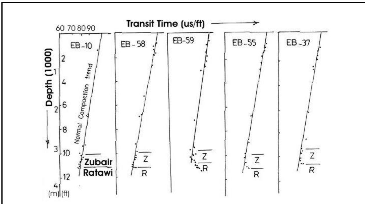
Fig. 6 : Shale transit time \Delta t with increasing depth in Zubair and Ratawi formations (wells 10, 58, 59, 55 and 37).
