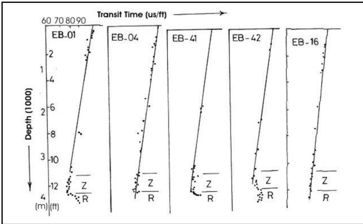
Fig. 7 : Shale transit time \Delta t with increasing depth in Zubair and Ratawi formations (wells 1, 4, 41, 42 and 16).
