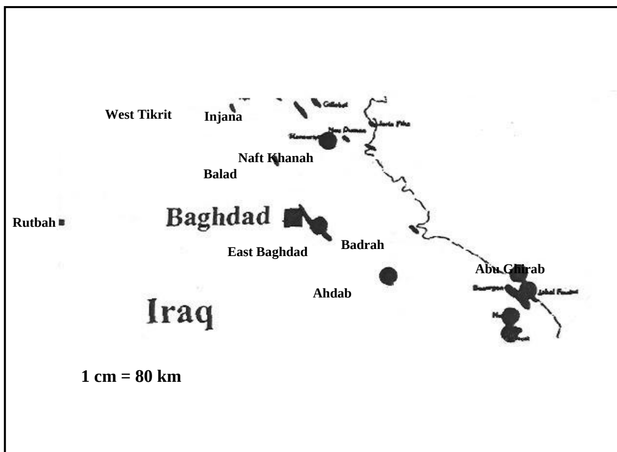
Fig.1 : Geographical location map of the studied area (1) .
