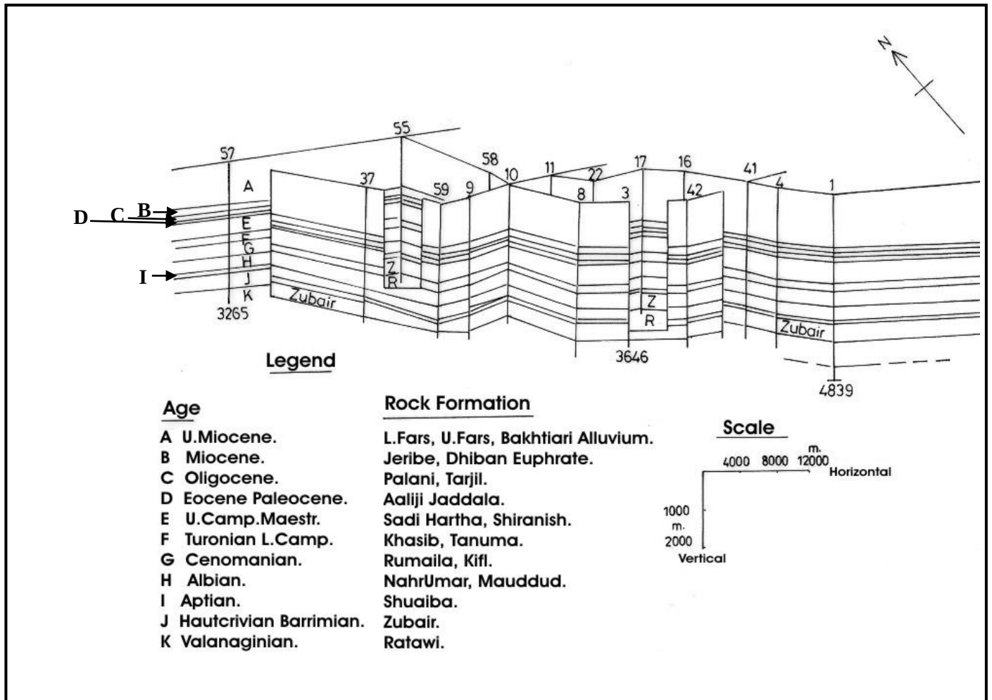
Fig. 4 : Panel diagram of East-Baghdad oilfield.
