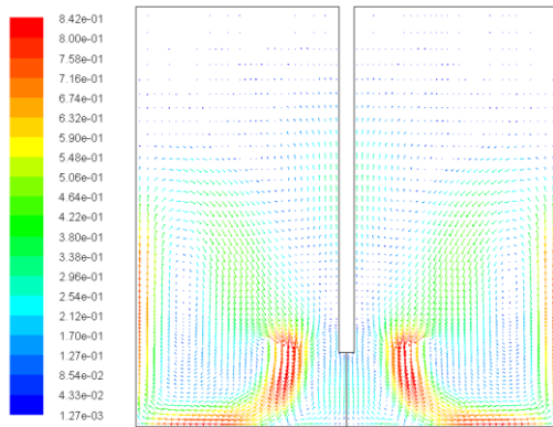
Figure 3 (c): Water velocity after 20 Sec. (m/s)
