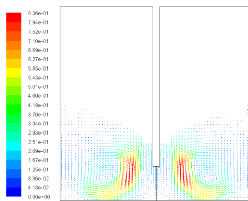
Figure 4 (a): Sand velocity after 1 Sec. (m/s)
