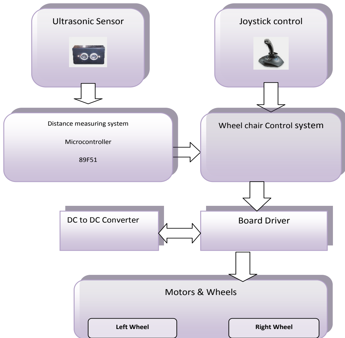
Fig.7. Control architecture of wheelchair
