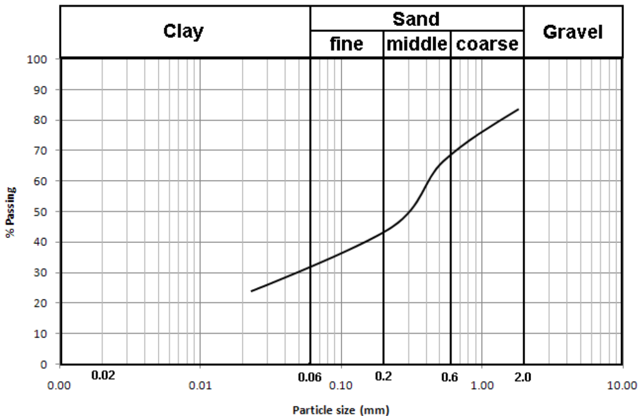
Fig 4 . Grain size distribution curve of bed material
