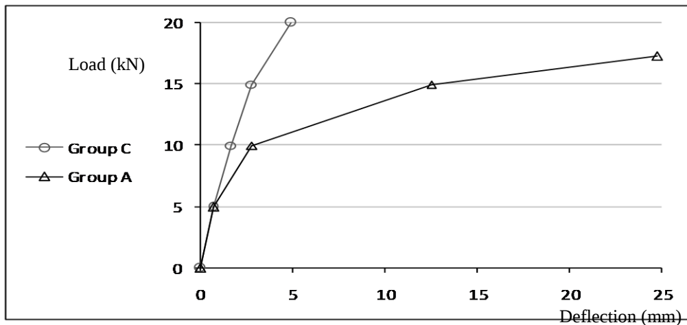
Fig 6 . Load – Deflection (P-Δ) relationship for panels in group (C) in comparison with the control specimens (group A)
