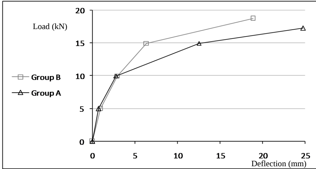
Fig 5 . Load – Deflection (P-Δ) relationship for panels in group (B) in comparison with the control specimens (group A)
