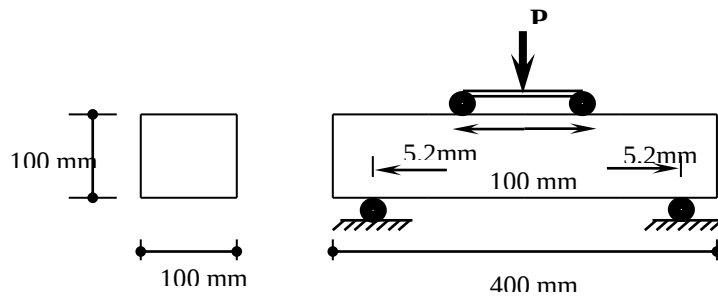
Fig. 2. Schematic diagram of the test setup for the beams prototypes during flexural investigation
