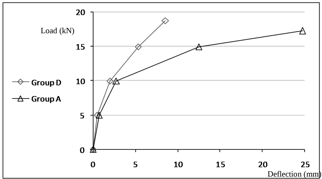
Fig 7. Load – Deflection (P-Δ) relationship for panels in group (D) in comparison with the control specimens (group A)
